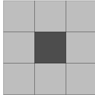
Figure 2: Queen neighbors (light) share either an edge or vertex (or both) with a reference spatial region (dark)[30]
