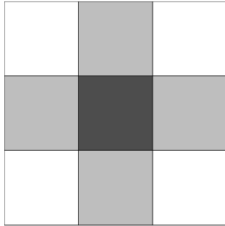
Figure 1: Rook neighbors (light) share an edge with a reference spatial region (dark)[30]
