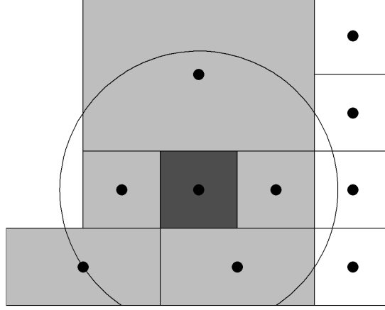
Figure 4: Distance-based neighbors (light) have centroids within a fixed radius of the reference cluster (dark). Clusters with centroids beyond this distance are not considered as neighbors (white)[30]
